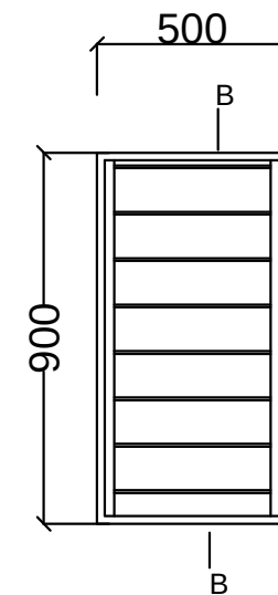
WINDOW TYPE W3 (LOUVERS)
