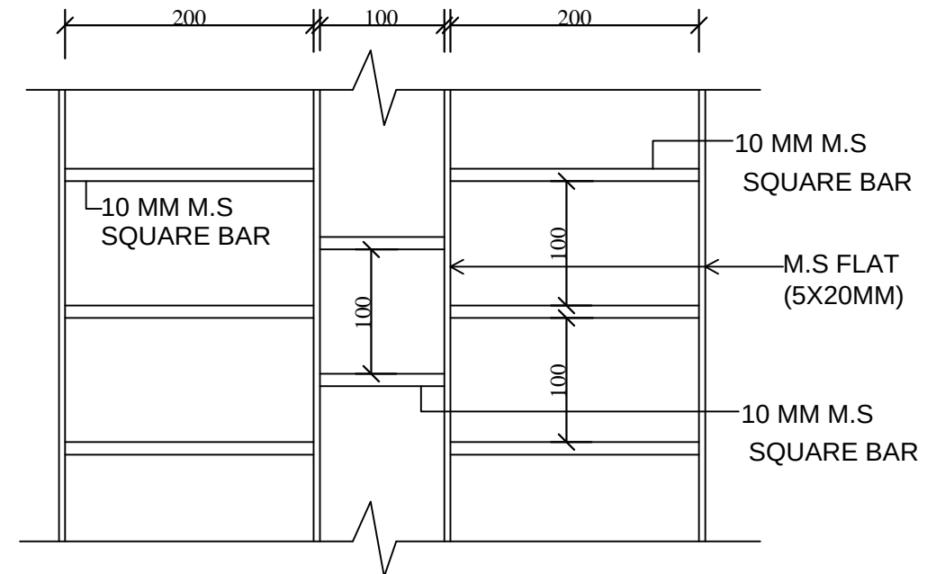
TYPICAL WINDOW AND VENTILATOR GRILL DETAIL
