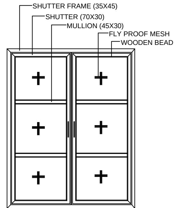
TYPICAL WINDOW AND VENTILATOR FLY PROOF DETAIL
